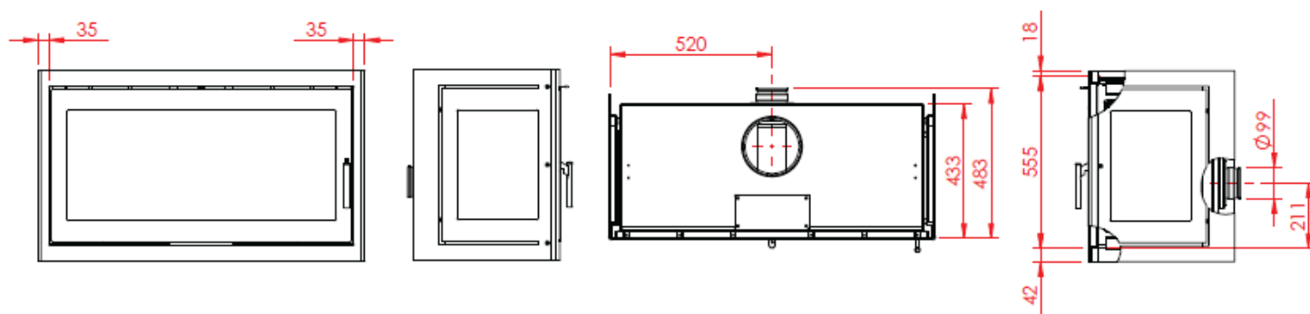
550 XXL fixed glass 2 sides, airbox behind
