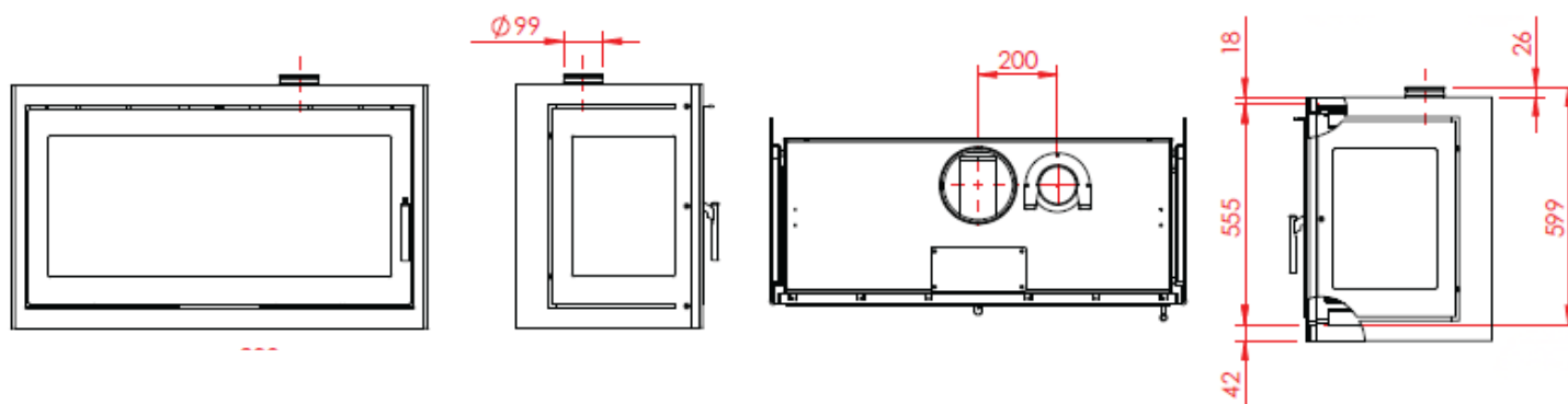
550 XXL fixed glass 2 sides, airbox on top
