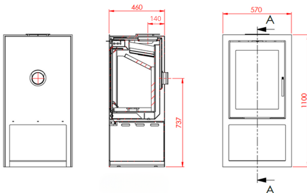
550 vertical with airbox and wood box
