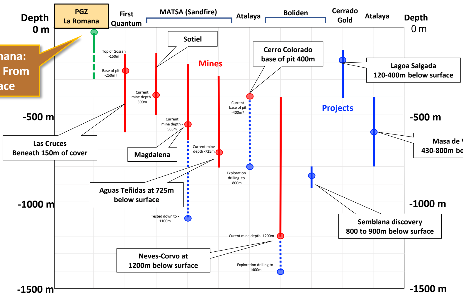
Iberian Pyrite Belt Deposits shown for comparison of drilling and mine depths. There is no assurance that Pan Global Resources' results will be similar or mirror those of adjacent properties.
