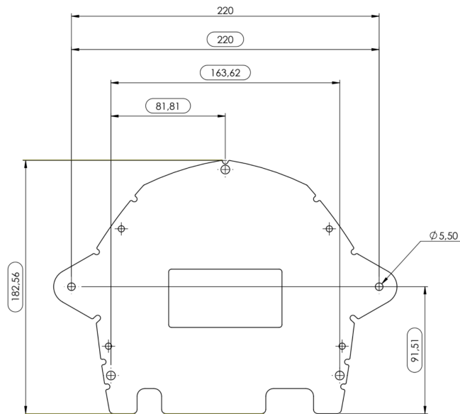
Figure 9: Smart Antenna Support Option 1 - Top View
