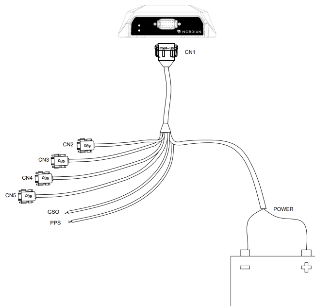
Figure 7: Connection Example
