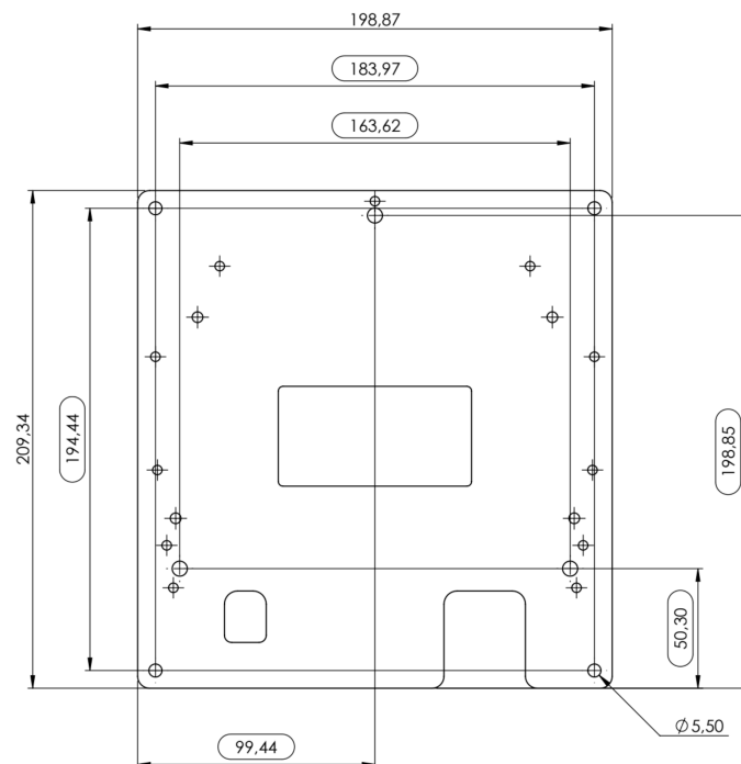
Figure 11: Smart Antenna Support Option 2 - Top View
