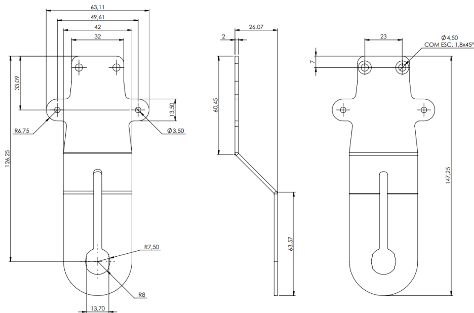
Figure 13: Ultra+ Antenna Support Dimensions (millimeters)
