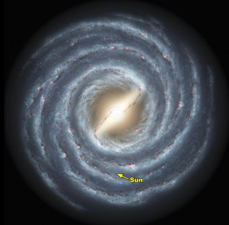
Milky way
