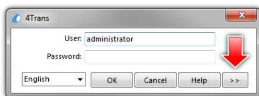
Fig. Button ">>"
