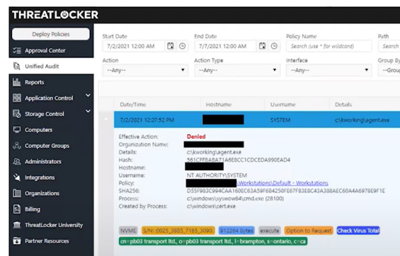
- Unified Audit showing c:\kworking\agent.exe being denied
