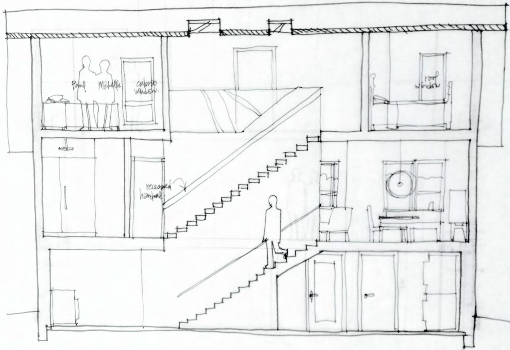
Lindsay Residence — DD section @ stair — Sept. 19.14.
