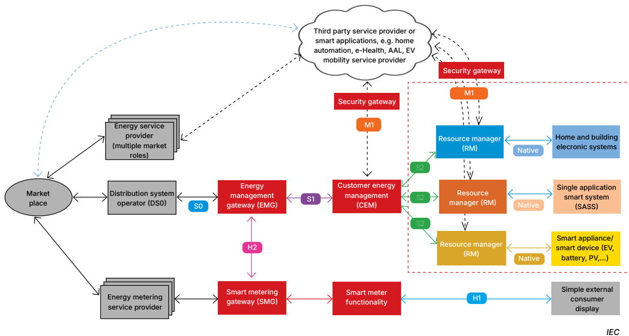
Figure 5 - Single CEM energy management architecture with a divided Actor B 1
