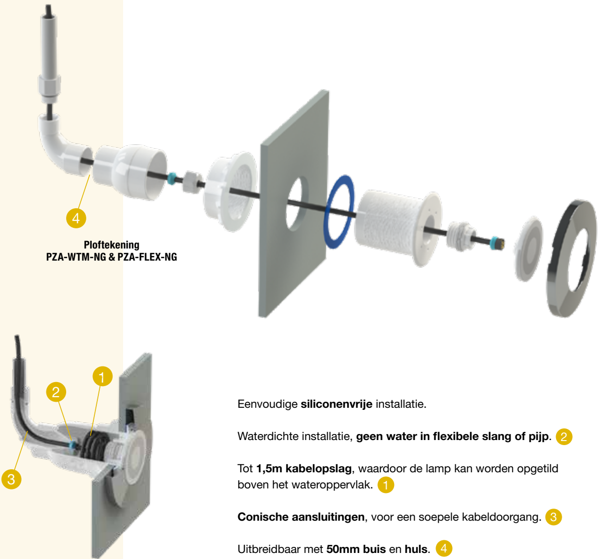
Dwarsdoorsnede PZA-WTM-NG & PZA-FLEX-NG
