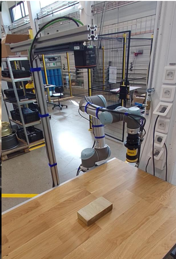
No Code Programming Mirka & IFM 3D Sensor
