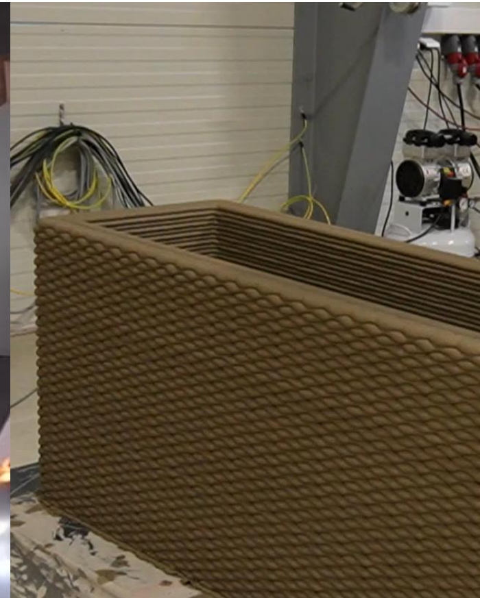
3D Concrete Printing
