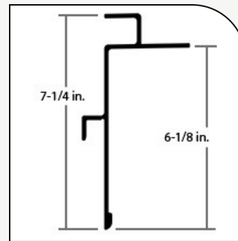
GDP60318848-30 BORDA SUPERIOR GD 30
