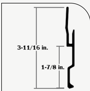
GDP60237971 X627 ZOCLO 627.5
