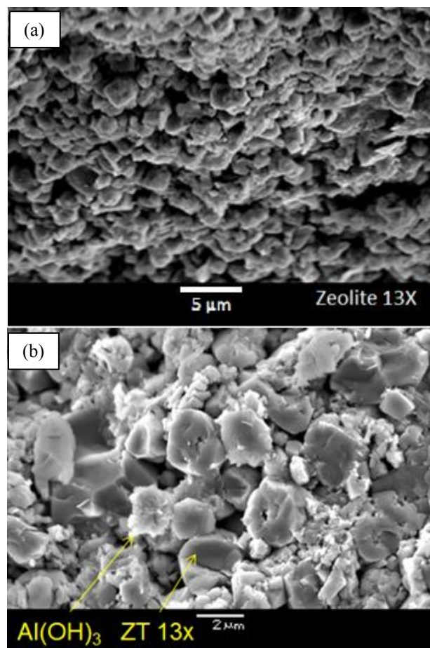
Figure 6. SEM images of (a) zeolite 13X and (b) zeolite 13X with 6.4wt.% \text{Al(OH)}_3
