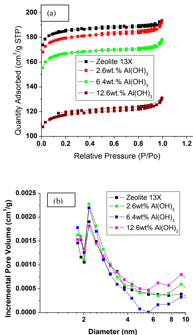
Figure 5. (a) Nitrogen adsorption isotherms and (b) pore size distribution of Zeolite 13X with and without \text{Al(OH)}_3 binder
