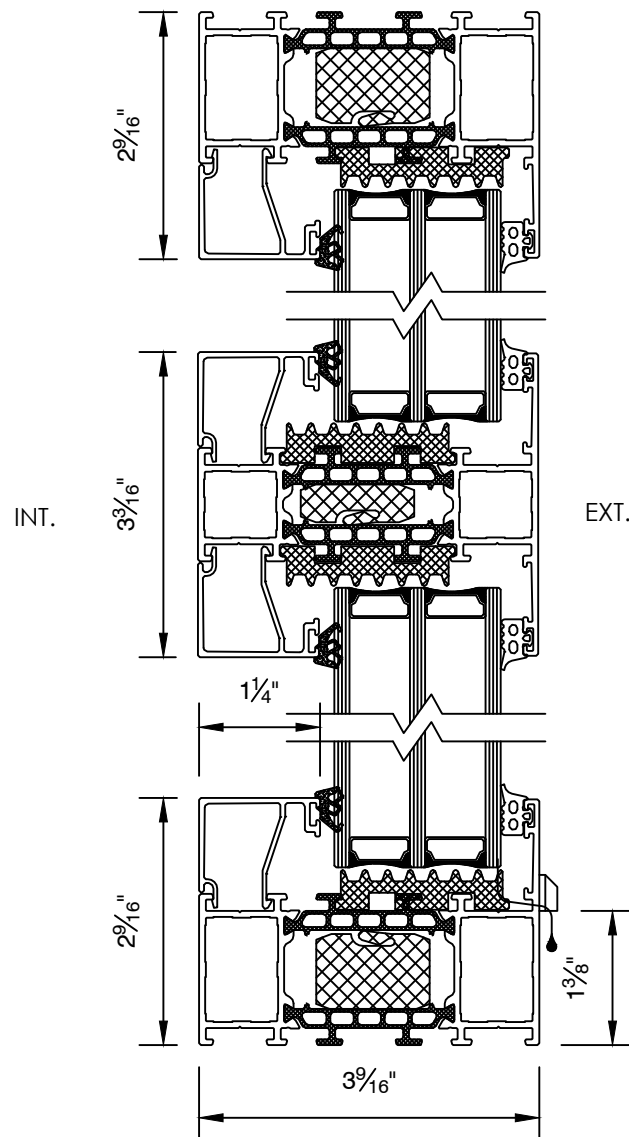
6 HEAD/SILL DETAIL SCALE: 6" = 1'-0"
