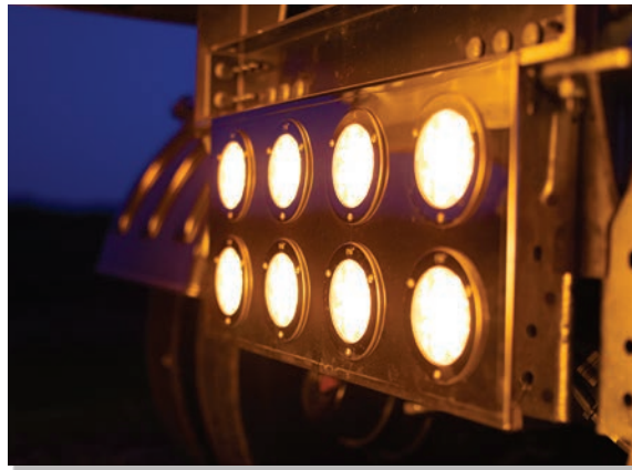
Forward facing bogie lights in a stainless steel box
