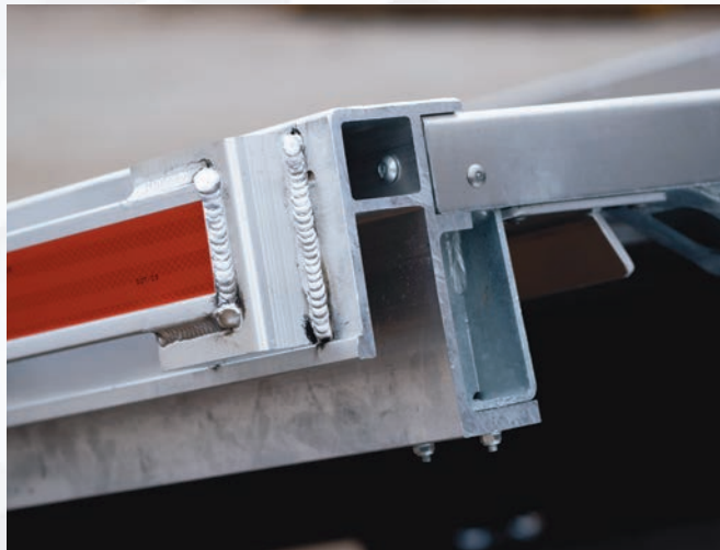
Eby Exclusive 7-1/2" x 4-5/8" Tilt Side Rail
