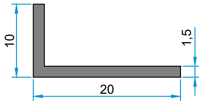
Angle 20x10x1.5mm
