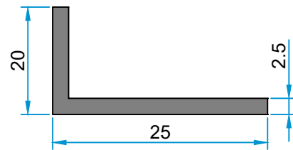
Angle 25x20x2.5mm
