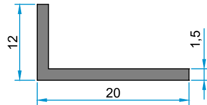
Angle 20x12x1.5mm
