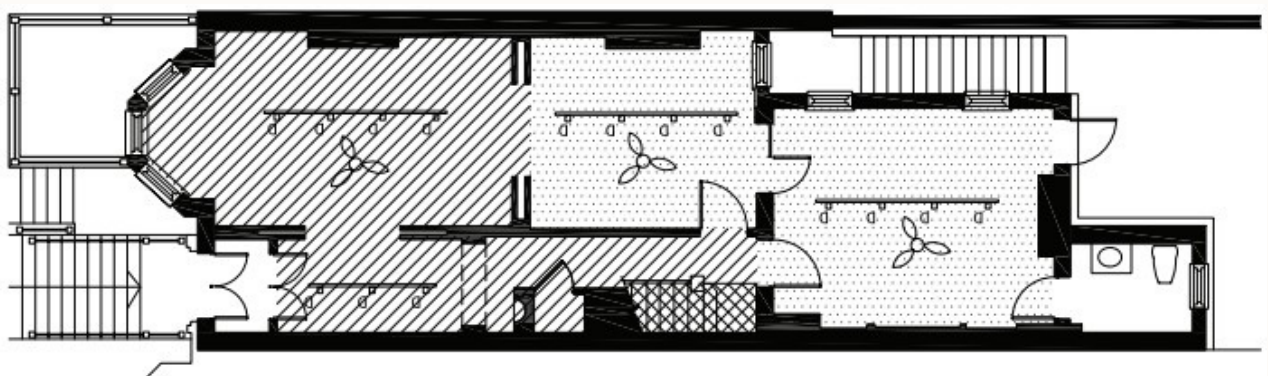
1 st Floor
