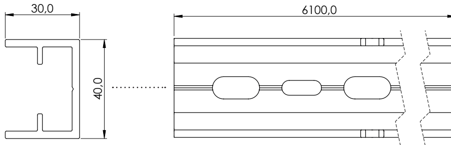
22284 Mounting rail
