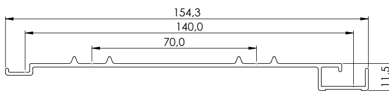
21263 Double profile 70
