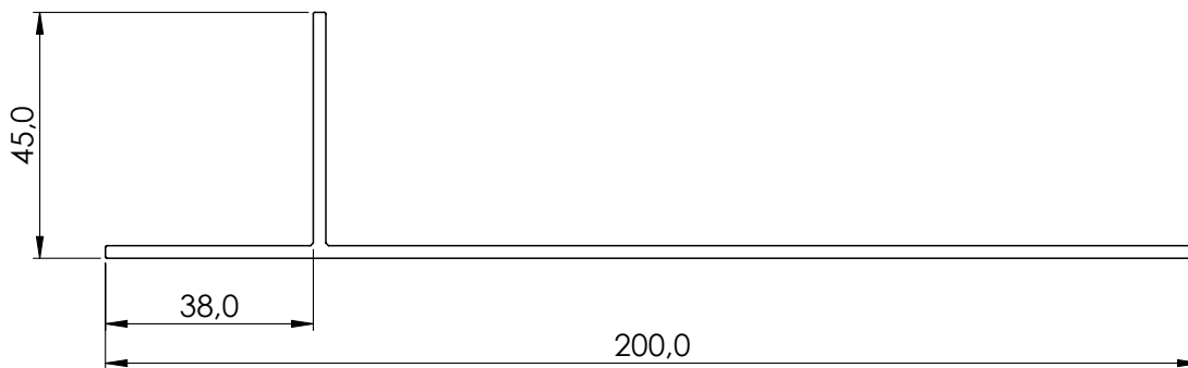
24167 Side and top rebate
