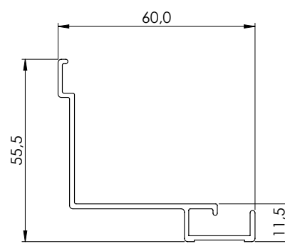
22394 Internal profile 70
