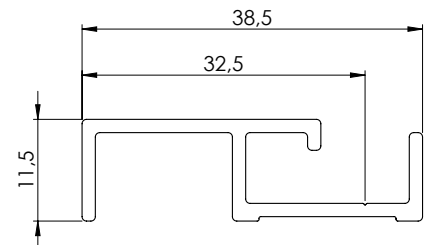
22914 Start profile 32,5
