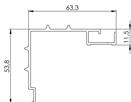
22912 External profile 58
