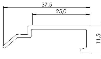
24170-X End profile 25
