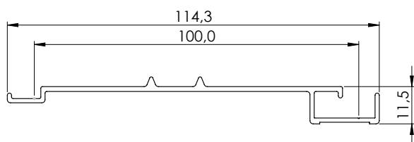
23171 Single profile 100
