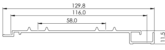
22911 Double profile 58
