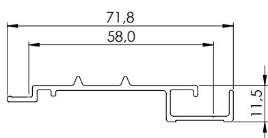
22910 Single profile 58
