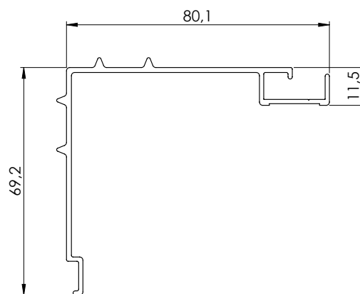
23855 External corner 100 and 34x34 mm lamella
