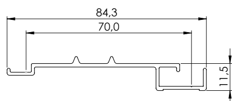
21264 Single profile 70
