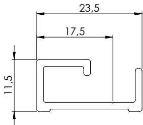
22953 Start profile 17,5
