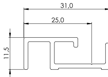
410 Start profile 25
