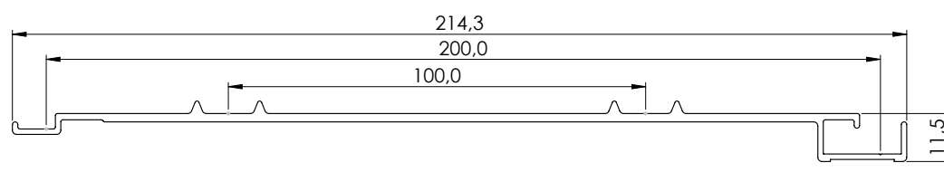
23170 Double profile 100
