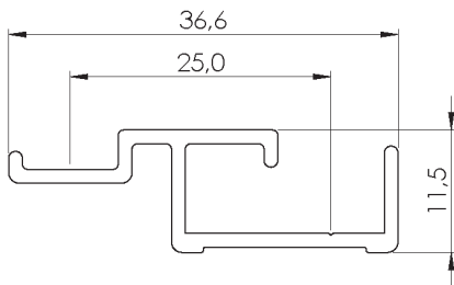
22926 Middle profile 25
