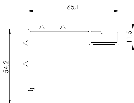
22136 External profile 70
