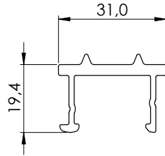
23115 Reinforced Woodfac profile
