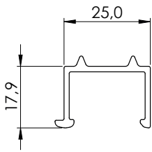
20707 Woodfac profile
