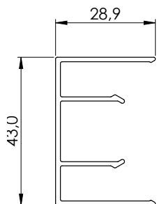
22680 Cover for mounting rail
