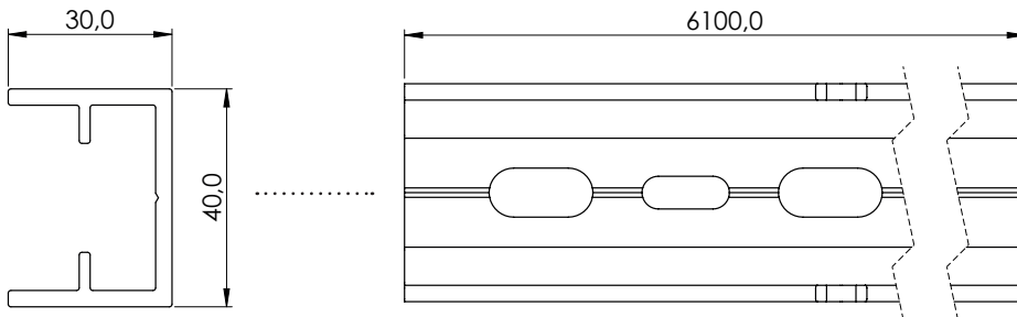
22284 Mounting rail
