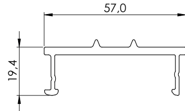
23060 Wide reinforced Woodfac profile
