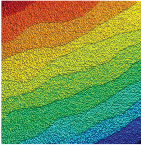
Topography of \text{SrTiO}_3 in dynamic mode. Scan size: 1 \times 1 \mu\text{m}^2 .
