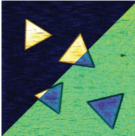
Topography (left) and KPFM signal (right) of CVD grown \text{MoS}_2 crystals. Scan size: 42 \times 42 \mu\text{m}^2 ; Z-range: 9 nm; KPFM range: 1.45 V.
