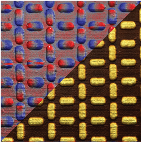
MFM and topography on artificial spin ice (data courtesy: Prof. S. Ferreira). Scan size: 4 \times 4 \mu\text{m}^2 .
