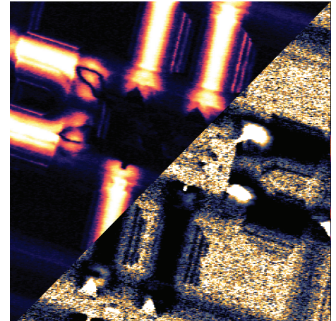
Amplitude (left) and phase (right) of dS/dV ( dC/dV ) measurement on SRAM sample. Scan size: 11 \times 11 \mu\text{m}^2 .
