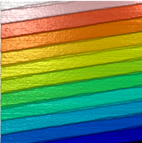
SiC steps Scan size: 1.5 µm x 1.5 µm The scan shows step heights of 1.5 nm between the large terraces, and 0.75 nm between the large and small terraces’ half-steps.
