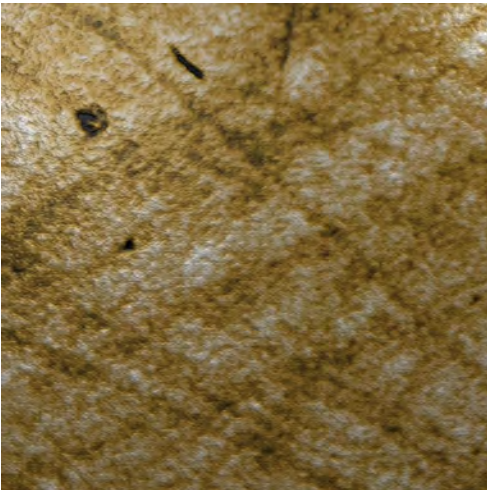
Glass Scan size: 5 µm x 5 µm Surface roughness: 0.112 nm RMS (0.087 nm Ra)
