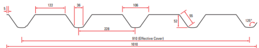
Maxispan Reverse Run (Optional but not standard) Dimensioned Drawings of Maxispan Reverse Run (For wall cladding only)
