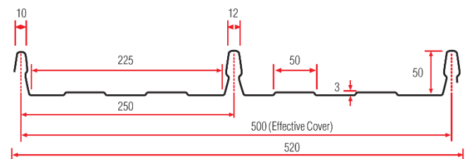
All dimensions are nominal, in mm. Sheet cover width tolerance +/-5mm.
