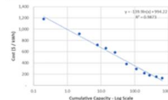
Li-ion Battery Costs vs Cumulative Capacity
