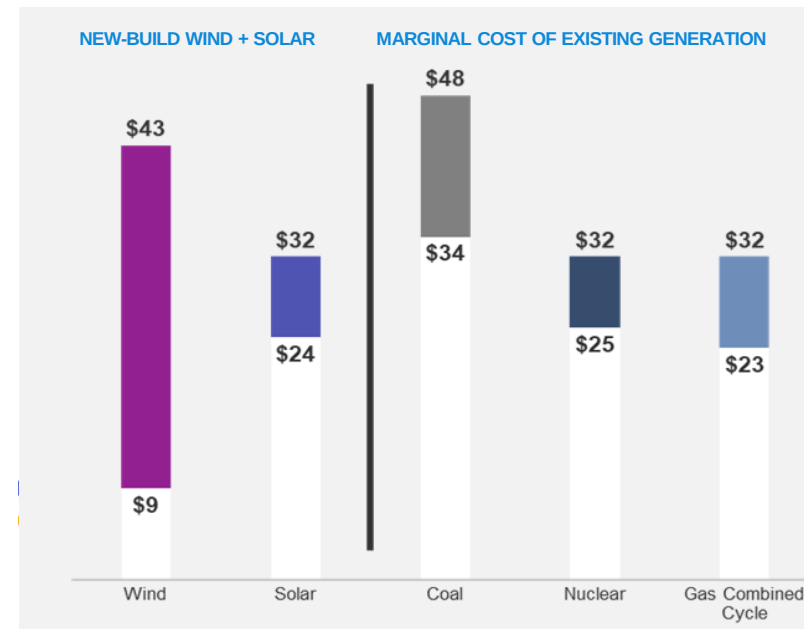
Levelized Cost of Electricity in 2020, $/MWh
