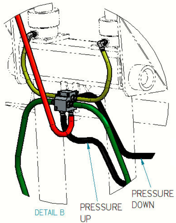
DETAIL B
