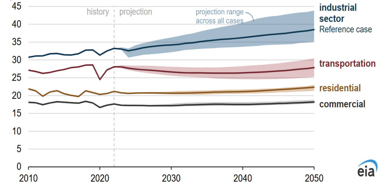
Total energy consumption by end-use sector, United States (2010–2050) quadrillion British thermal units
