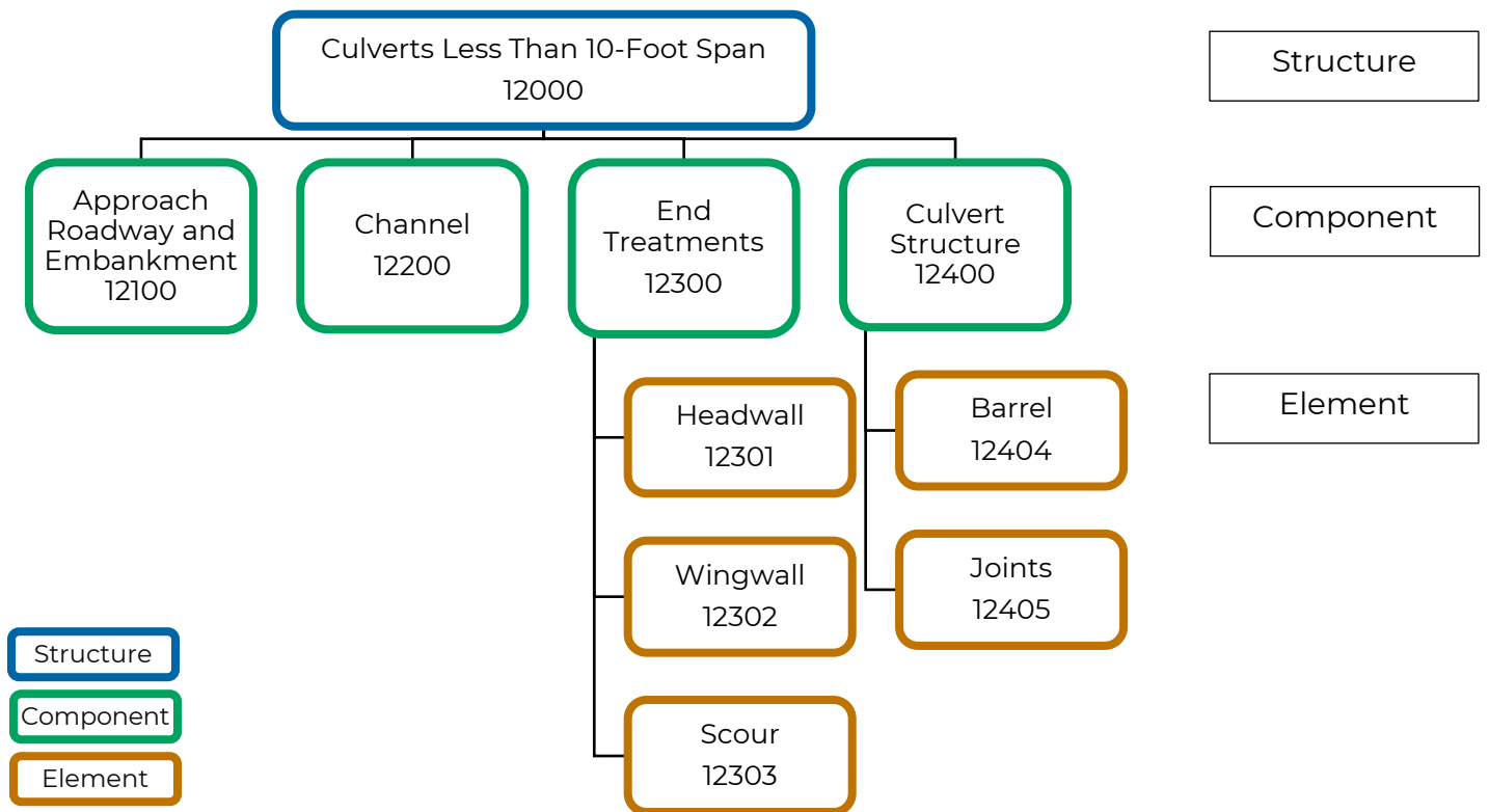
Figure 2-1: Component-element Structure for Culverts Less than 10-Foot Span
