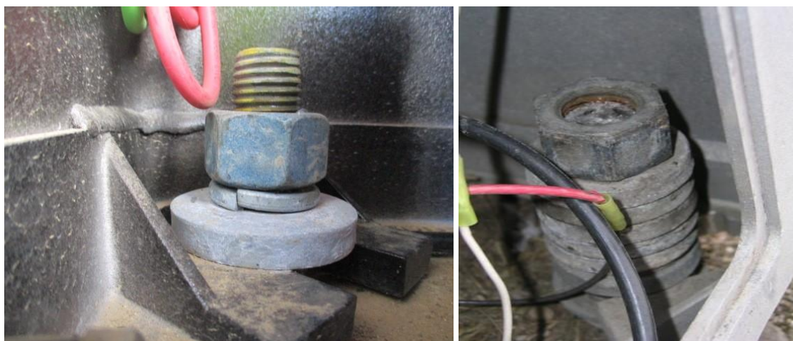
Figure 11-9: Frangible pole structure anchor bolts and leveling nuts foundation, loose anchor bolt (left), anchor nut without fully engaged thread (right)
