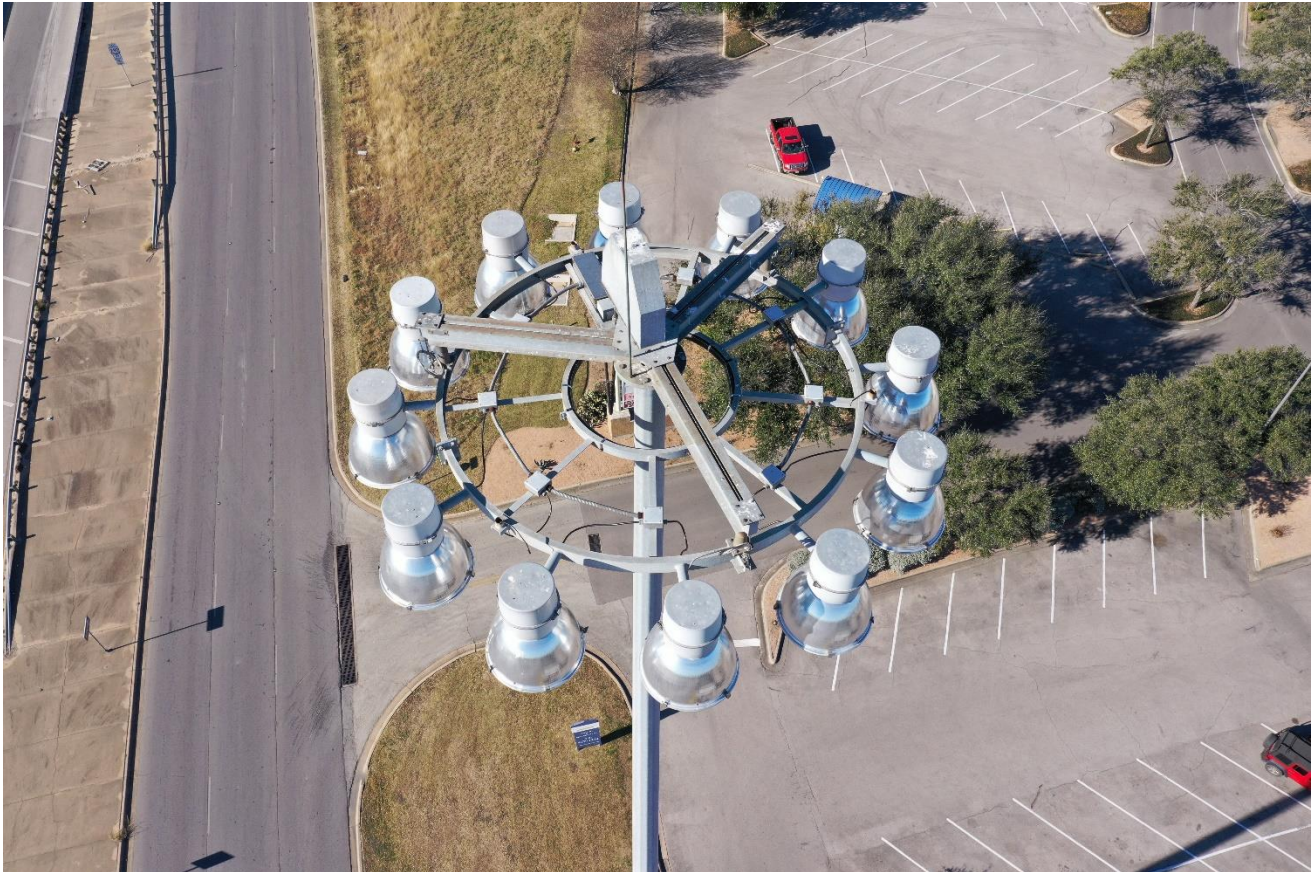
Figure 12-3: High-Mast Lighting Tower, aerial view of tower and lighting array from UAS
