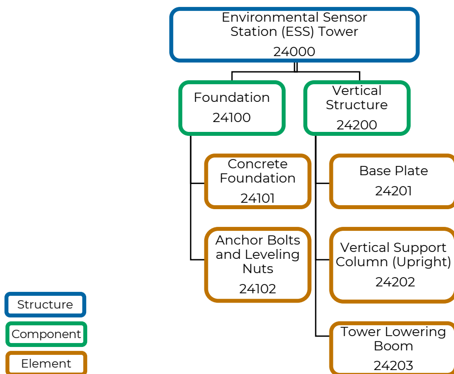
Figure 14-2: Elements and components for ESS Tower (adapted from MDOT Standards ITS-052-B, ITS-053-A)
