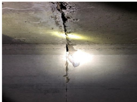
Figure 2-33: Spalling within a box culvert
