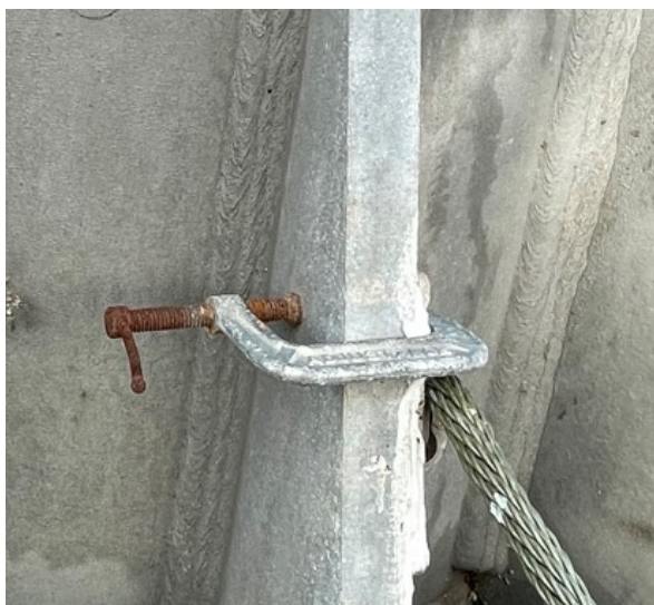
Figure 10-10: Corrosion in bonding clamp along bolt of base plate stiffener
