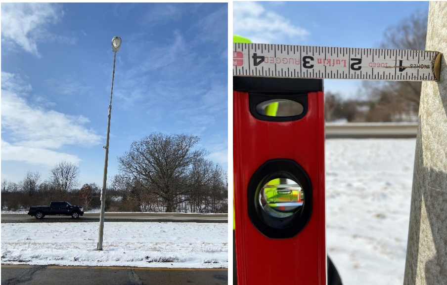
Figure 11-21: Non-frangible pole structure vertical support column (upright), visual identification of out of plumb pole (left), measurement of pole plumbness (right)
