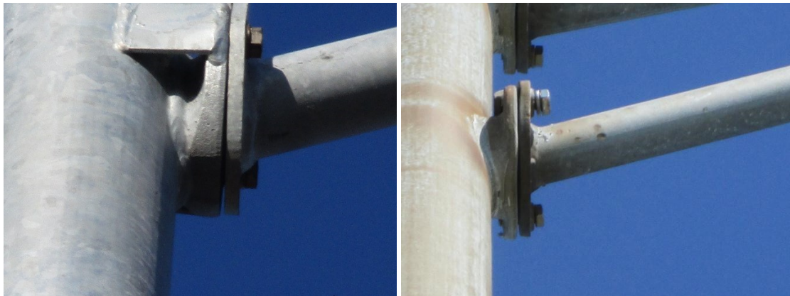
Figure 11-22: Frangible and non-frangible pole structure vertical structure connections, gap at arm flange (left), loose arm connection bolt (right)
