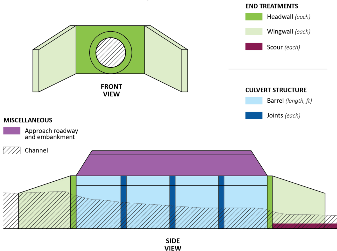
Figure 2-3: Elements and components for Culverts Less Than 10-Foot Span Culverts Less Than 10-Foot Span
