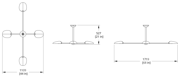
PT-4SS Pilot Chandelier Single Tier Dimension
