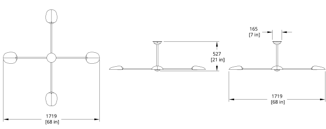
PT-4SL Pilot Chandelier Single Tier Dimension
