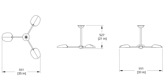
PT-4SL Pilot Chandelier Single Tier Dimension
