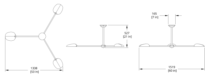
PT-4A Pilot Chandelier Single Tier Dimension
