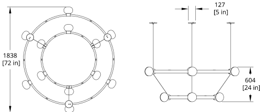
C64-66 Cinema Chandelier Dimension
