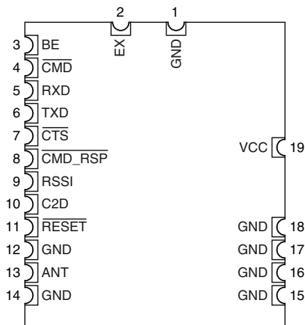
Figure 5: 25 Series Transceiver Pin Assignments (Top View)
