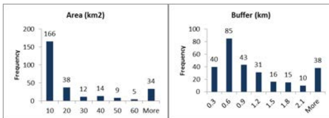
Figure 14: Histograms of area distribution (left) and buffer width zone distribution (right) for the 278 reservoirs impounded after 1993
