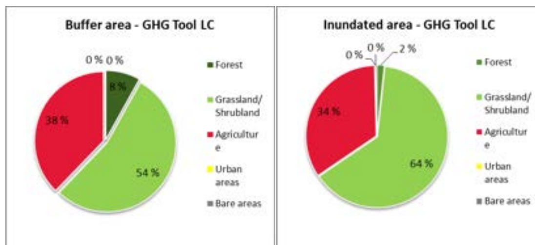
Figure 22: LC distribution for the Three Gorges Reservoir determined in the buffer area (left) and in the inundated area (right). LC categories from the GHG Screening Tool. The land cover with "water" use is not included
