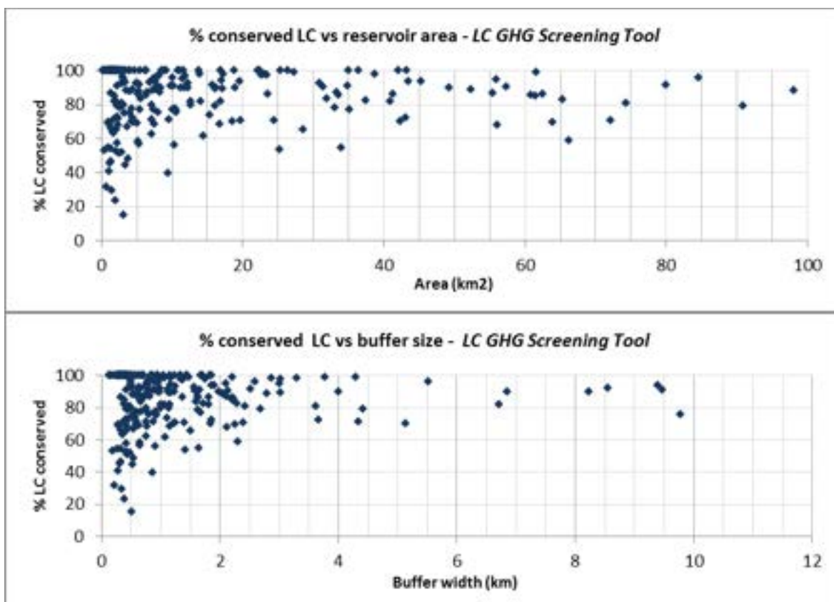
Figure 15: Percentage of conserved LC as a function of reservoir area (upper) and buffer size (lower)
