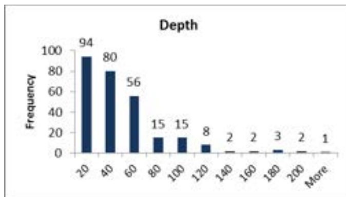
Figure 19: Histogram of depth distribution for the 278 reservoirs impounded after 1993
