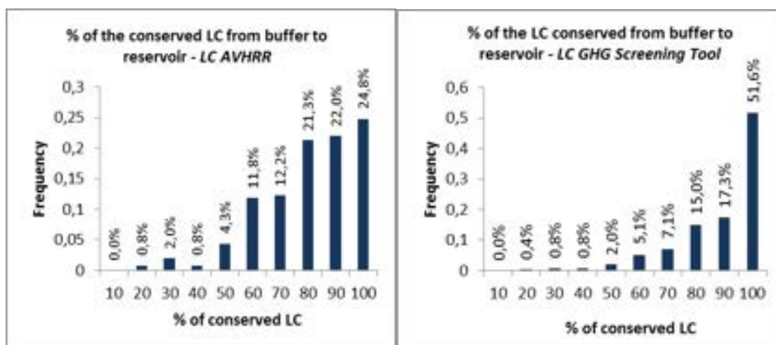
Figure 13: Percentage of Land Cover conserved from the buffer area to the reservoir area for the AVHRR land cover categories (left) and for the GHG Screening Tool LC classes (right)
