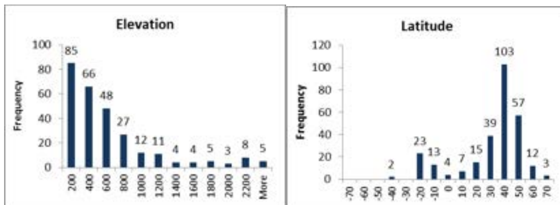
Figure 16: Histograms of elevation distribution (left) and latitude distribution (right) for the 278 reservoirs impounded after 1993
