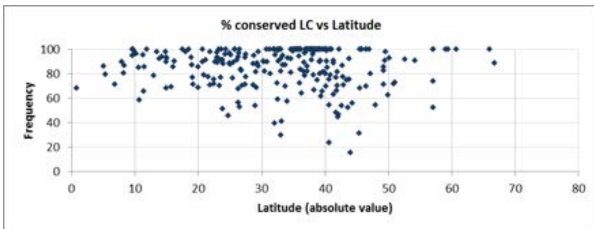
Figure 18: Percentage of conserved LC as a function of reservoir latitude. Latitudes are set to positive values
