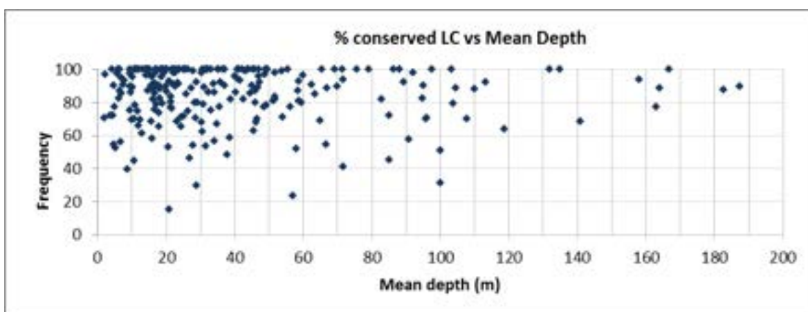
Figure 20: Percentage of conserved LC as a function of reservoir mean depth
