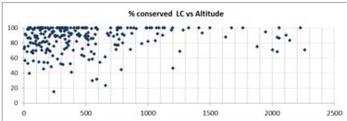
Figure 17: Percentage of conserved LC as a function of reservoir altitude
