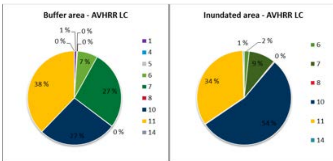
Figure 21: LC distribution for the Three Gorges Reservoir in the buffer area (left) and in the inundated area (right). LC categories satellite data. The land cover type "water" use is not included
