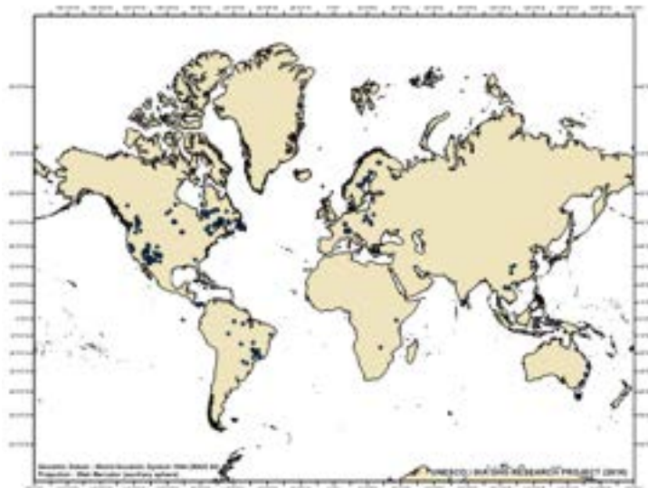
Figure 3: Location of the 223 reservoirs with \text{CO}_2 and \text{CH}_4 emissions data from the actual and past scientific literature used in the modeling
