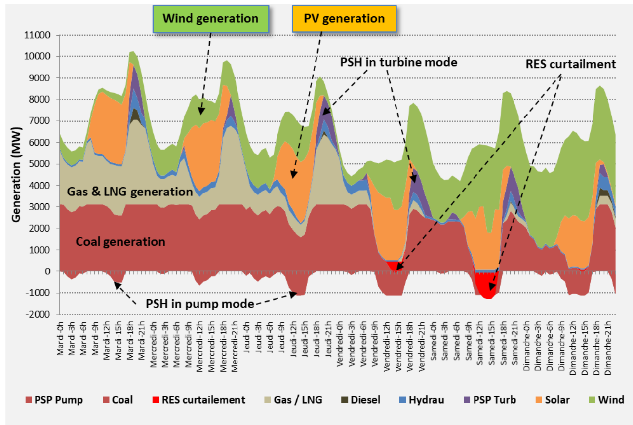
Figure 8. Projection of a 6-day load-generation balance in Morocco by 2025 assuming 30% of solar and wind penetration rate. "Hydrau" in the legend refers to hydro power not including PSH. (12)
