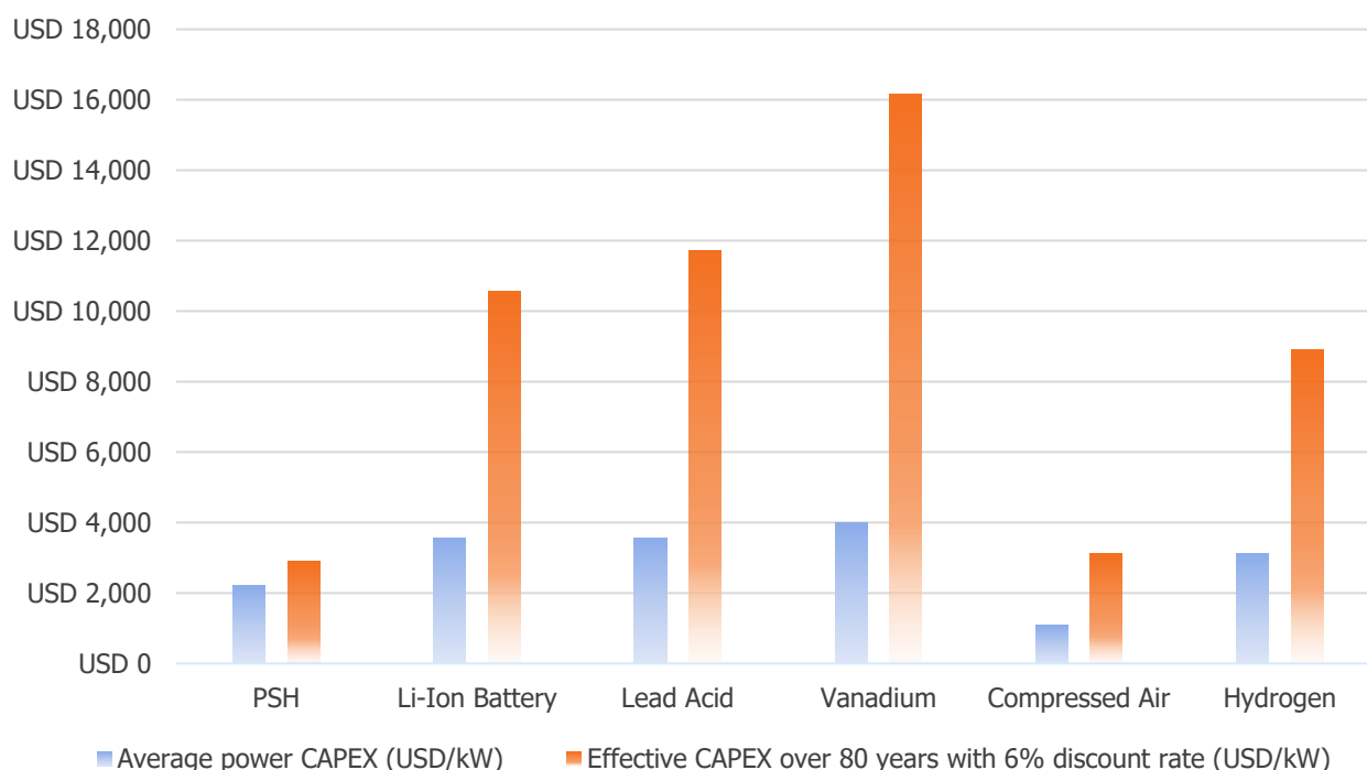
Figure 5. Comparison of effective lifetime costs of energy storage technologies over 80 years (10-hour duration, 2020)
