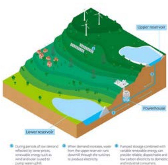
Figure 1. Illustration of a pumped storage hydropower plant
