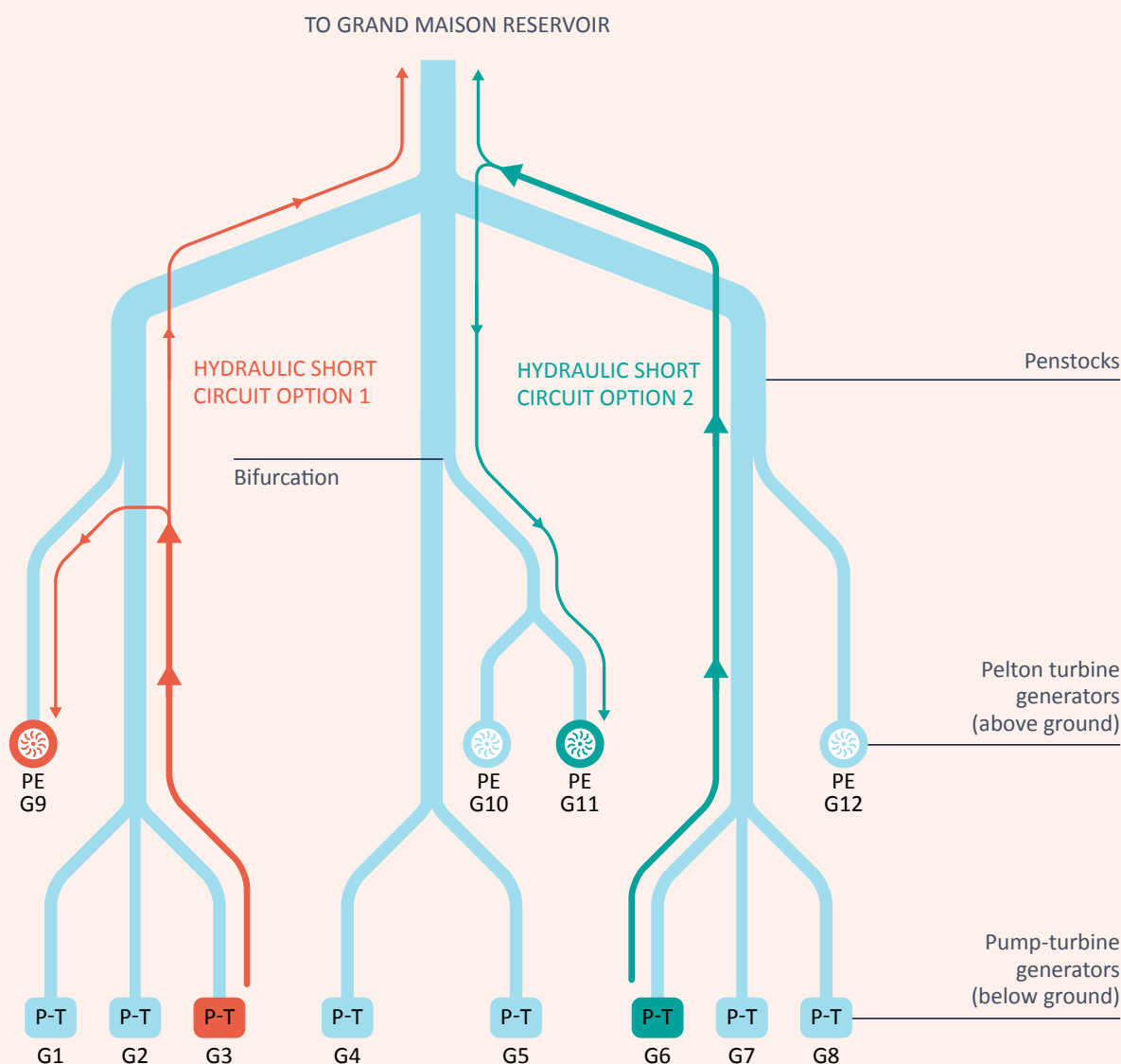
Figure 14: Illustration of the hydraulic short circuit options
