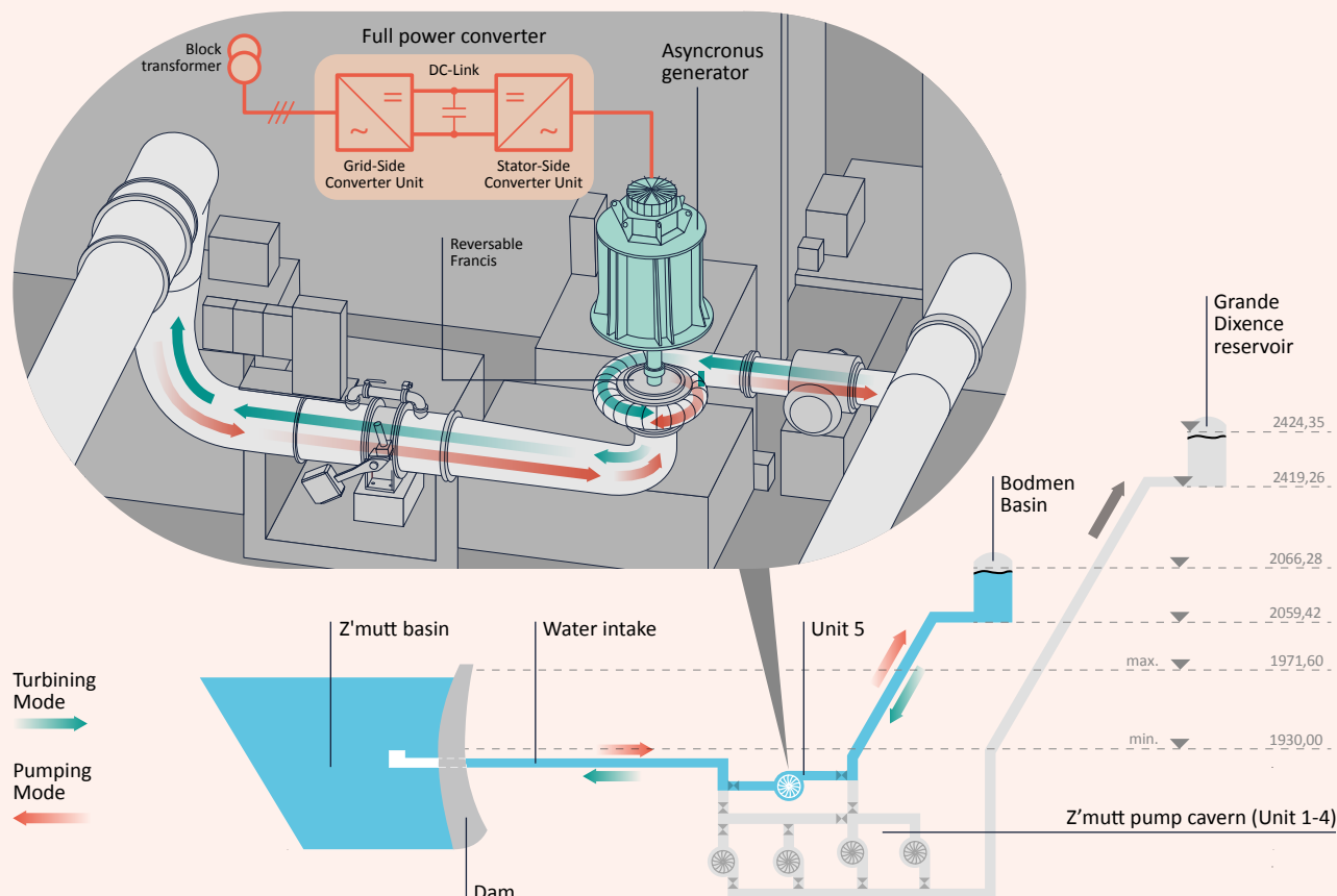
Figure 16: Z'Mutt unit 5 - location and connections to reservoirs
