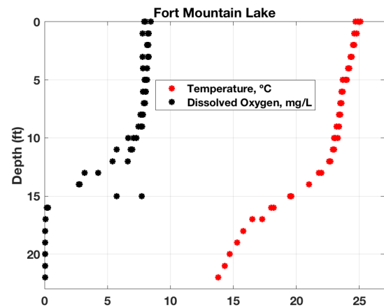
Figure 1. Water quality profile of Fort Mountain Lake in North Georgia (3 Sept 2015).
