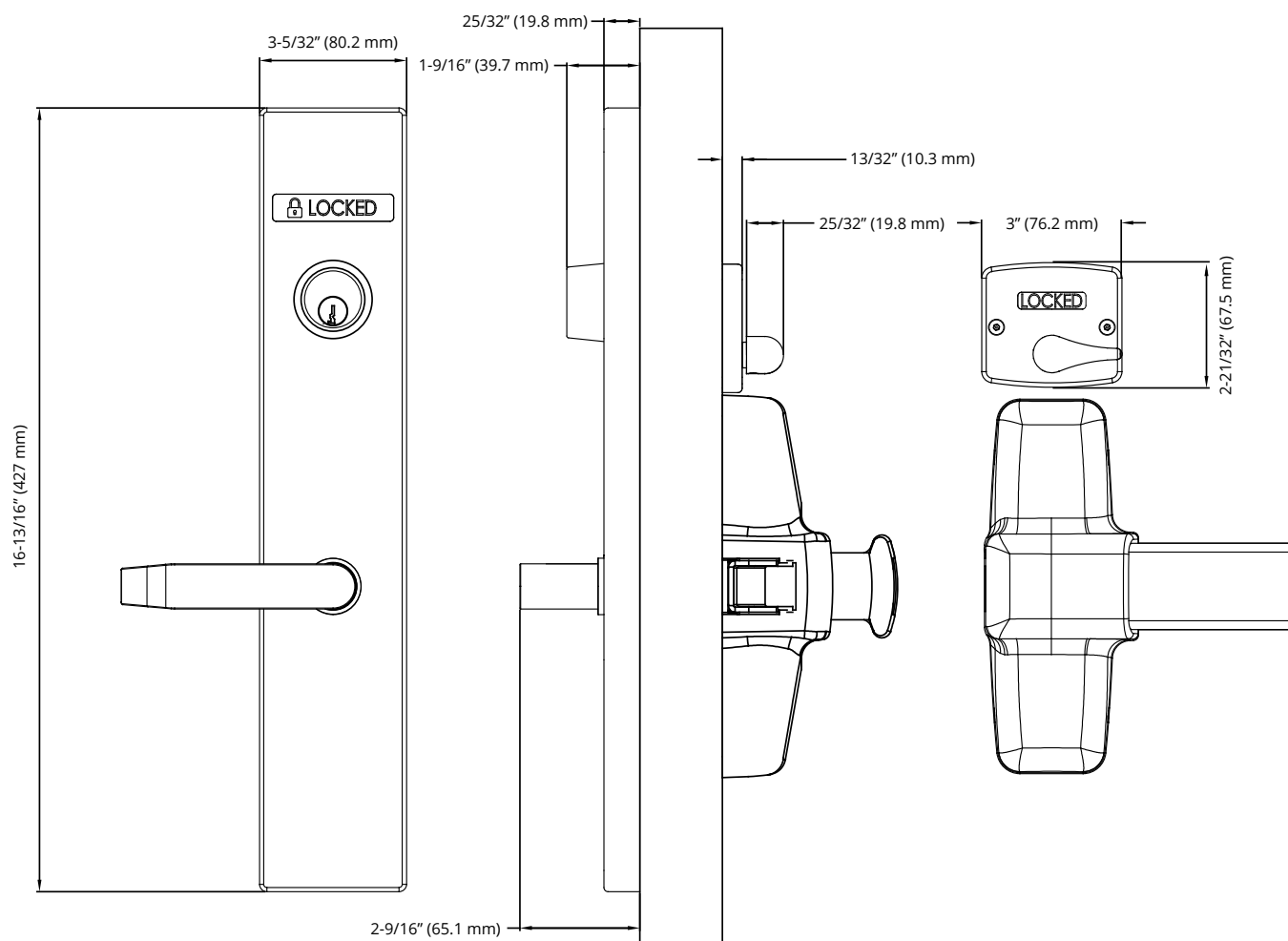
Rim device format, ESG F08T (Entrance) function, left hand reverse shown (Note: Exit device not included)
