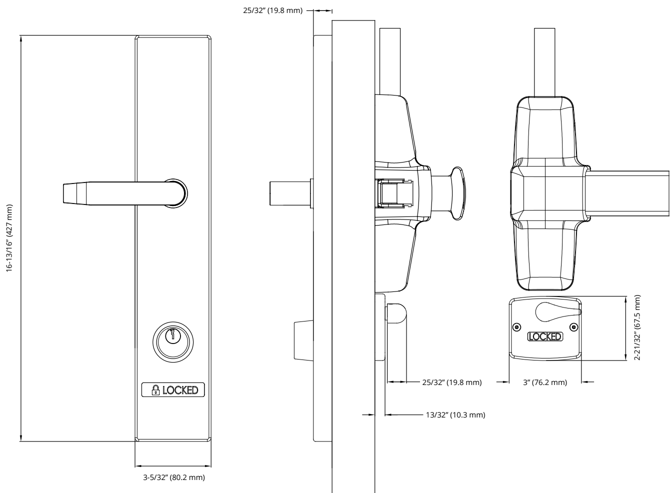
SVR LBR device format, ESG-LBR F08T (Entrance) function, Sentinel lever, left hand reverse shown (Note: Exit device not included)
