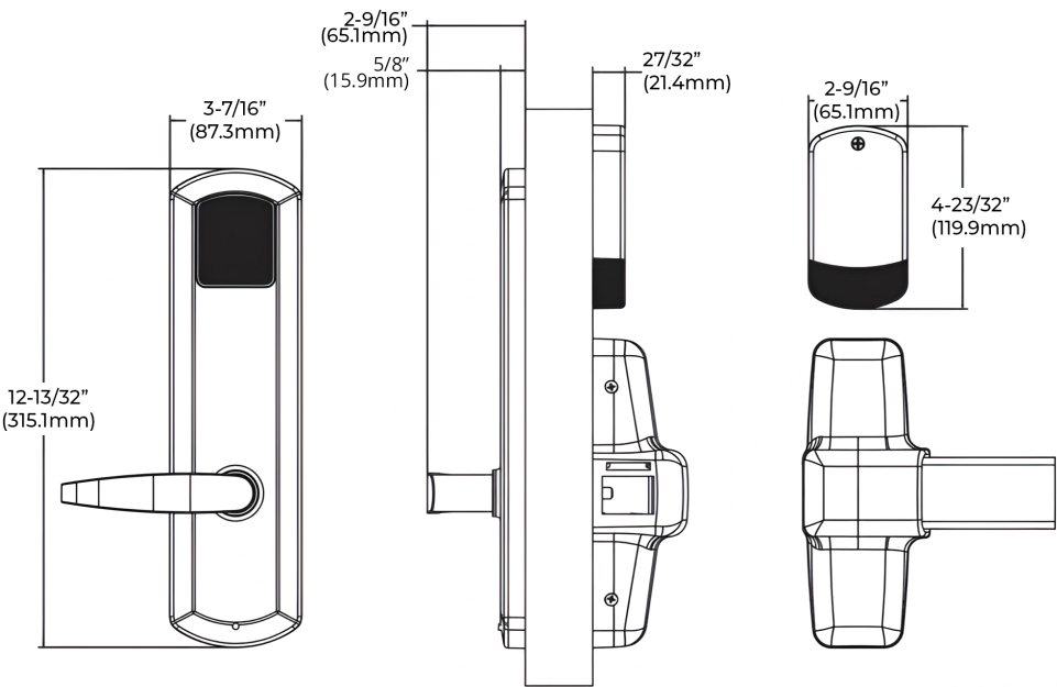
EKE Electronic 7000 1A without cylinder, Quest lever, left hand reverse shown (Note: Exit device not included)
