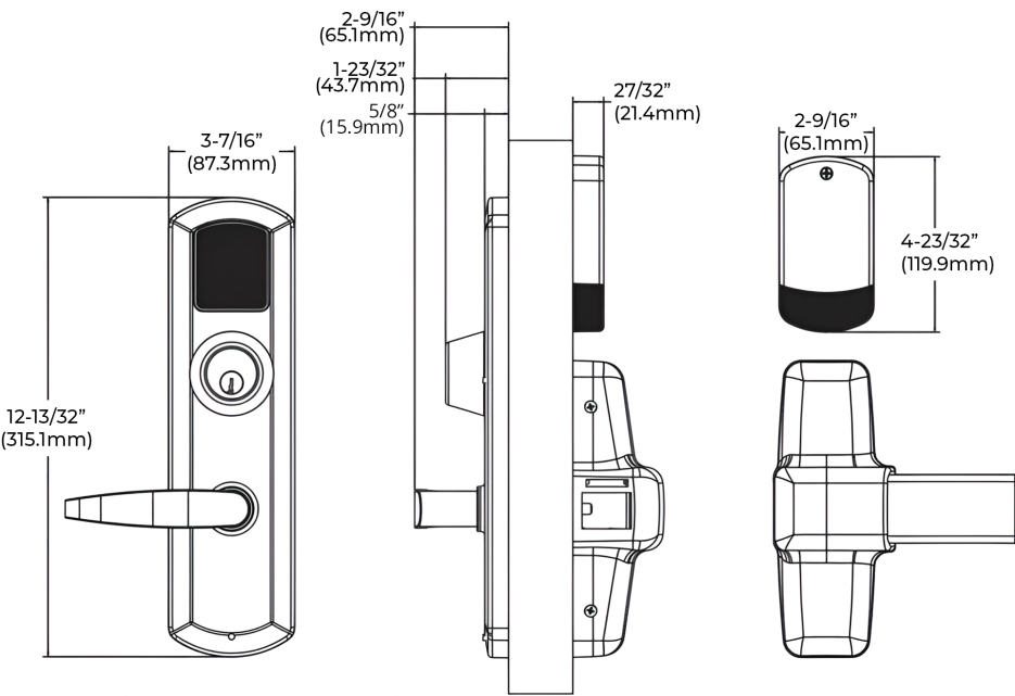
EKE Electronic 7000 1B with cylinder, Quest lever, left hand reverse shown (Note: Exit device not included)
