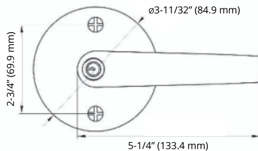
ED8900LQ F08 (Entrance) function shown
