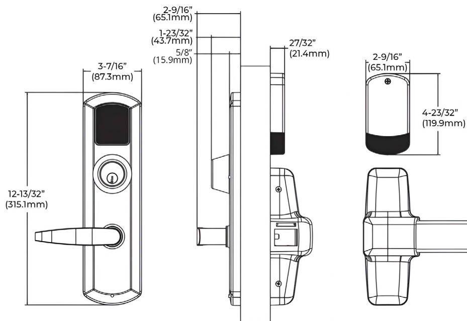
EKE Electronic 5000 1B with cylinder, Quest lever, left hand reverse shown
