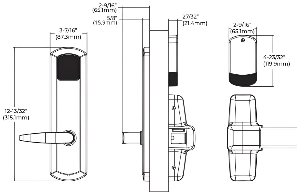
EKE Electronic 6000 1A without cylinder, Quest lever, left hand reverse shown (Note: Exit device not included)
