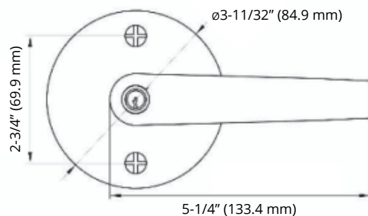
ED8900LS F08 (Entrance) function shown
