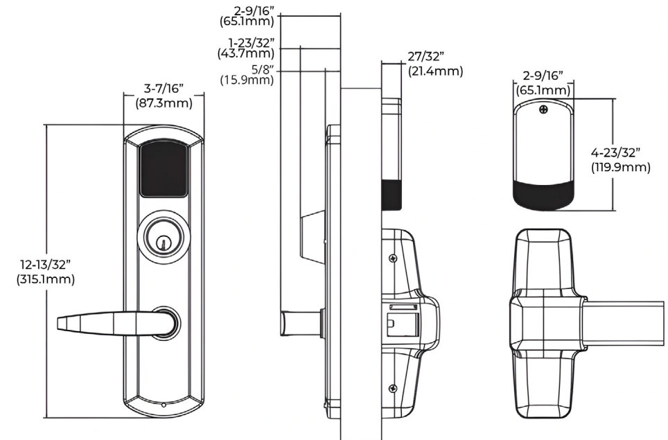
EKE Electronic 6000 1B with cylinder, Quest lever, left hand reverse shown (Note: Exit device not included)
