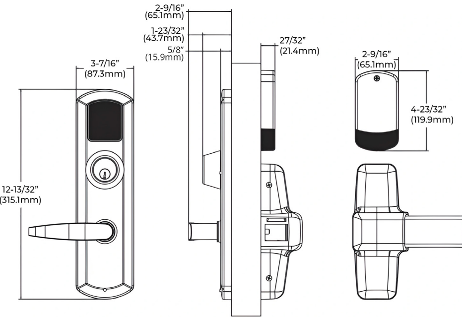
EKE Electronic 4000 1B with cylinder, Quest lever, left hand reverse shown (Note: Exit device not included)
