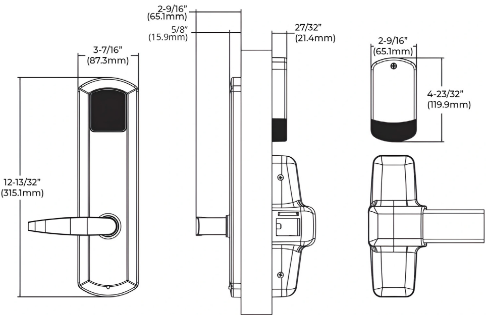
EKE Electronic 4000 1A without cylinder, Quest lever, left hand reverse shown (Note: Exit device not included)
