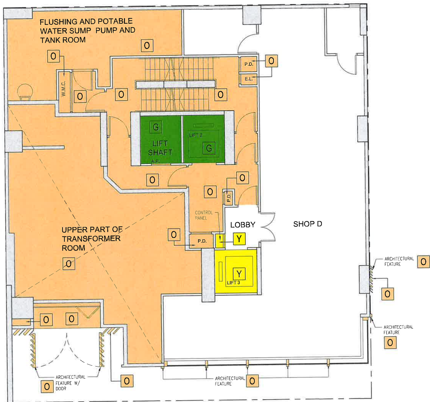
2/F FLOOR PLAN
