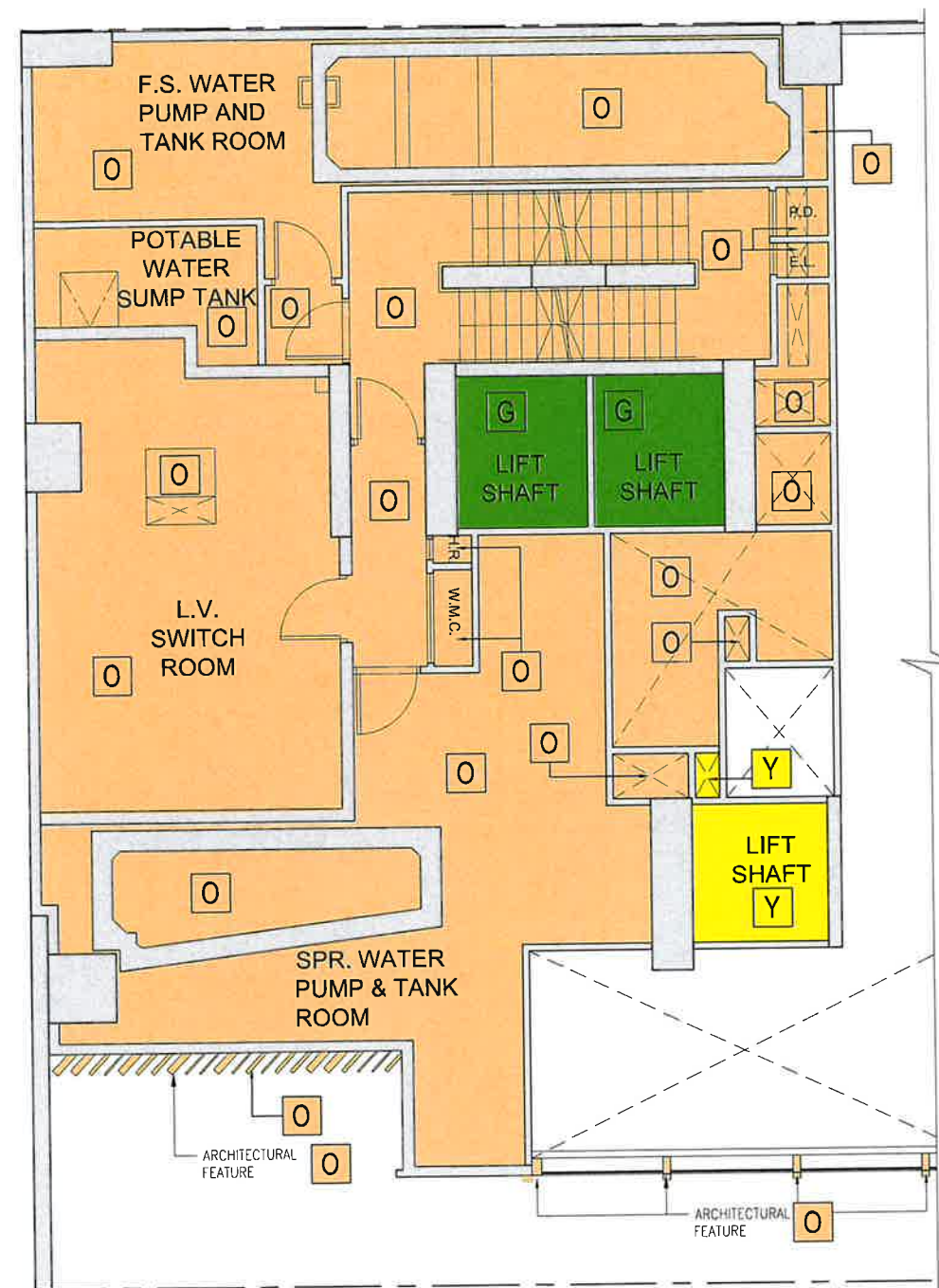
2/F FLOOR PART PLAN
