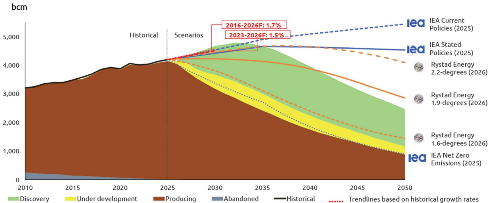
Figure 3: Global natural gas supply gap under various demand degree scenario
