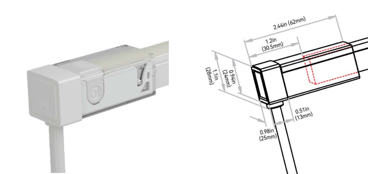
SIDE LEFT EXIT: 7-C-#
