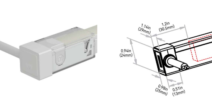
SIDE RIGHT EXIT: 7-D-#
